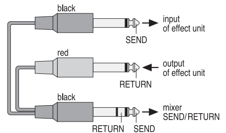
⑥ Connection of the MONACOR Y-cable MCA-202
